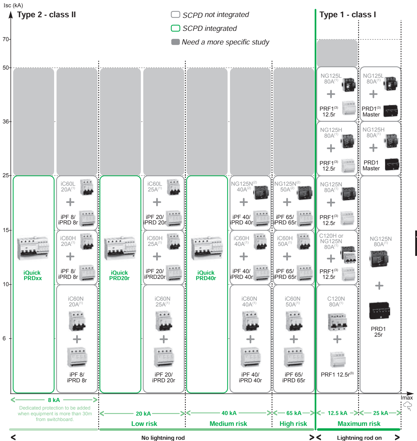
Fig. J37 : Coordination table between SPDs and their disconnecting circuit breakers of the Schneider Electric brand (1): All circuit breakers are C curve - (2): NG 125 L for 1P & 2P - (3): Also Type 2 (class II) tested
