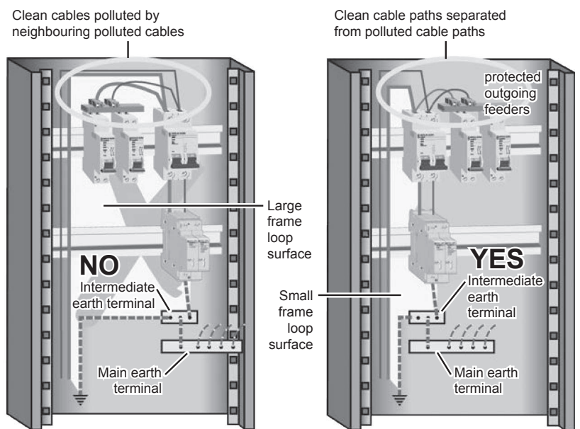
Fig. J42 : Example of improvement of EMC by a reduction in the loop surfaces and common impedance in an electric enclosure
