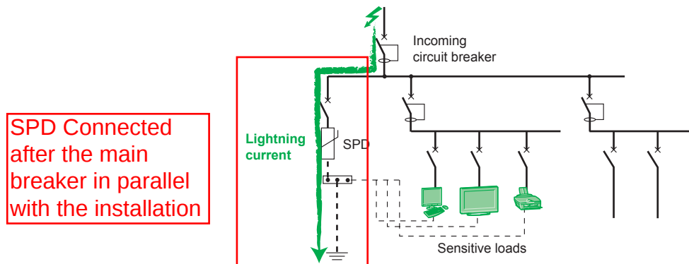
Fig. J17 : Principle of protection system in parallel
